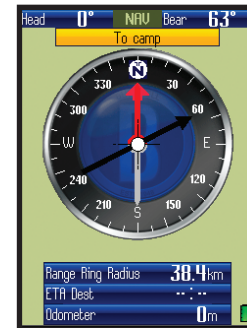
Fig 11. NAV Page
