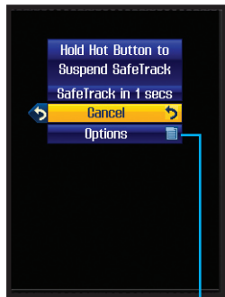
Fig 27. SafeTrack Screen
