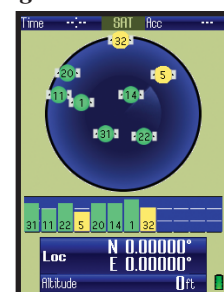
Fig 17. SAT Page
